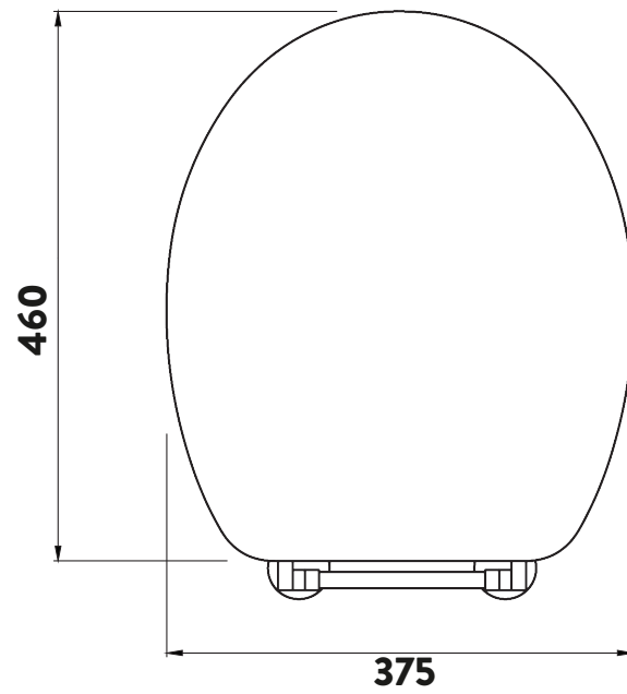
Overall Size
