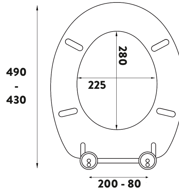
Max/Min Adjustment
